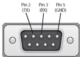
CA0052-M2T3R DB9 Male (Crossover)
