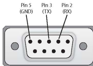
CA0052-F3T2R DB9 Female (Straight)
