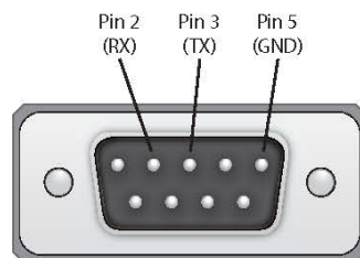
CA0052-M3T2R DB9 Male (Straight)
