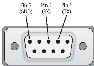
CA0052-F2T3R DB9 Female (Crossover)
